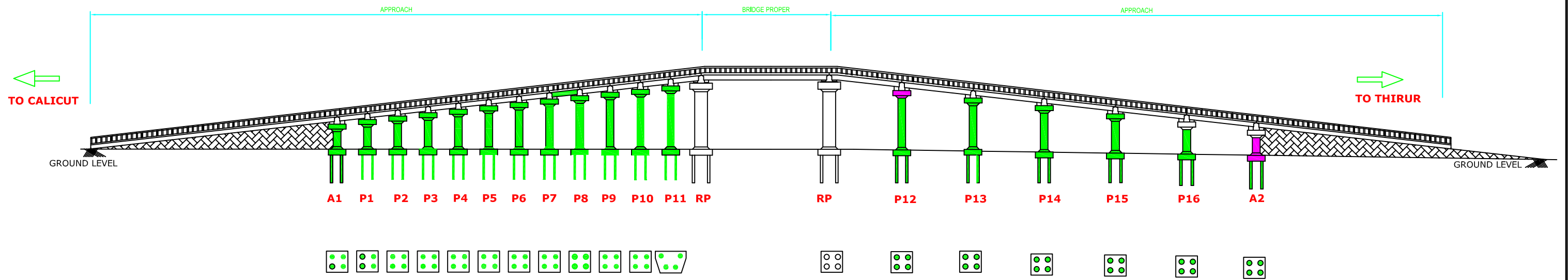
PILE FOUNDATION
